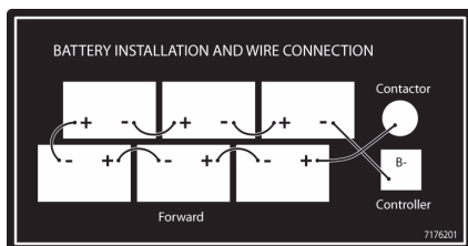
Battery Connection Decal
